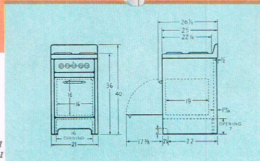
Dimensions of ER-541 and ER-501
