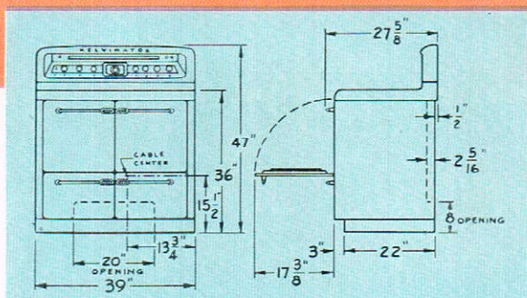
Dimensions of ER-509 and ER-507
