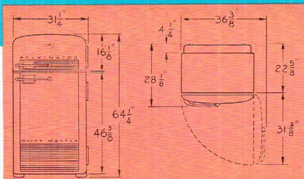
Dimensions of Masterpiece Model TM
