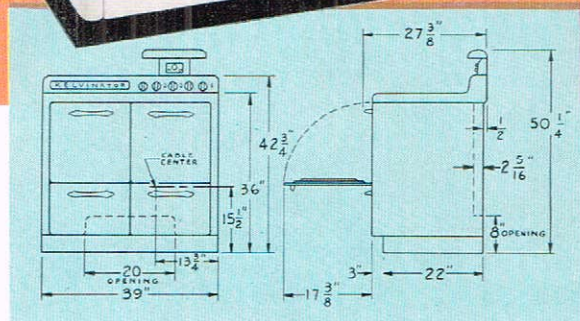
Dimensions of ER-503. Di- mensions of ER-502 are identical.
