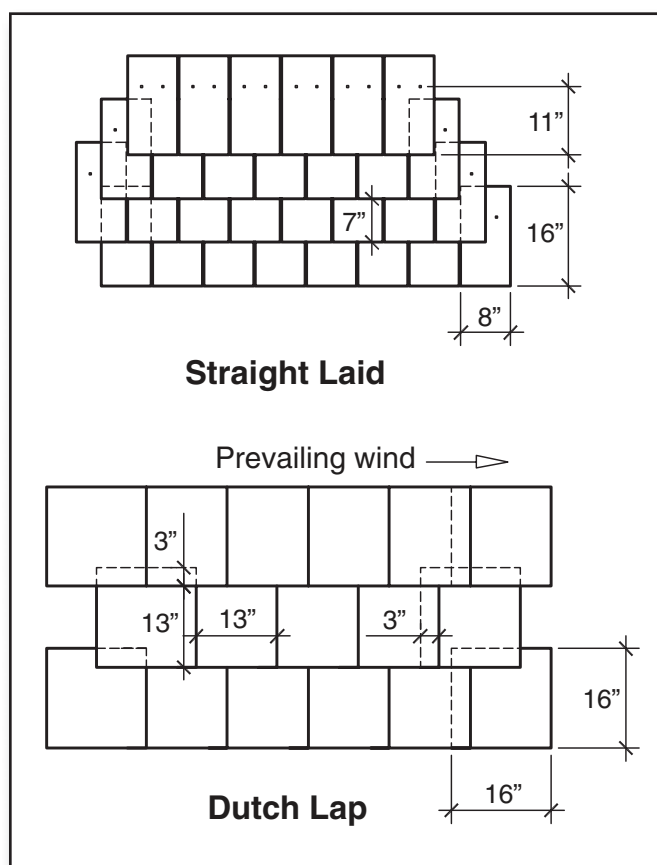
Figure 2—This drawing shows typical sizes, shapes, and installation for American method asphalt shingle roofing.
