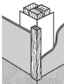
External Corner
