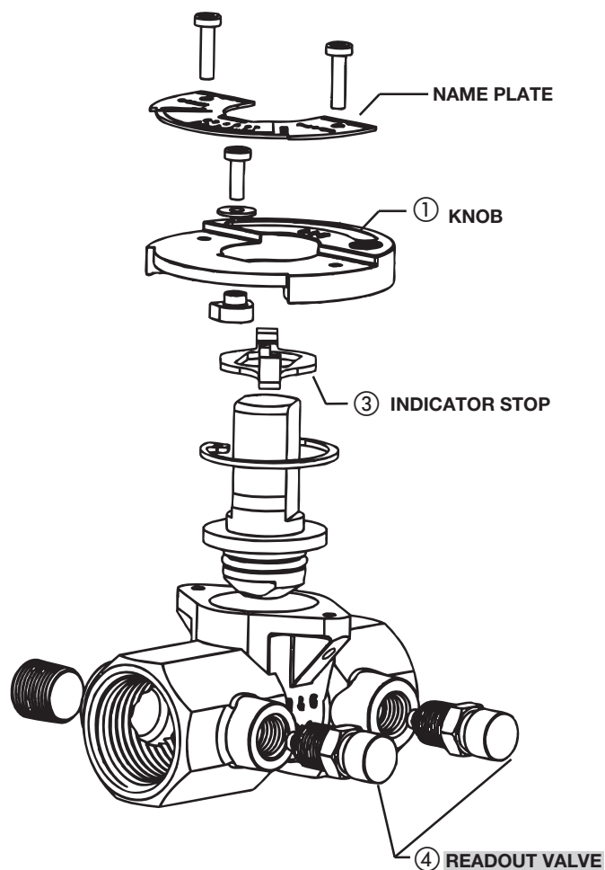
LARGE DESIGN BALL STYLE VALVE 1 1/4" – 3"
