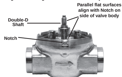
Fig. 4 - Shaft Position
