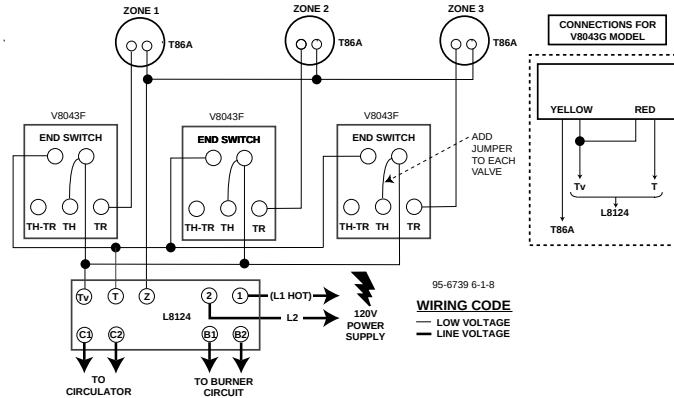
Fig. 6 - 3-ZONE SYSTEM USING L8124G AQUASTAT RELAY INTERGAL VALVE TRANSFORMER
