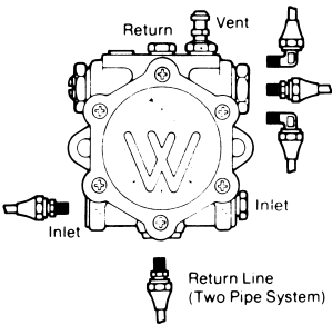
Standard A Style Installation: One or Two Pipe System
