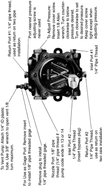
BODY STYLE D CLOCKWISE ROTATION BODY STYLE C COUNTERCLOCKWISE ROTATION (CCW) OPPOSITE OF THAT PICTURED
