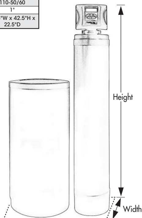
CSP Model
