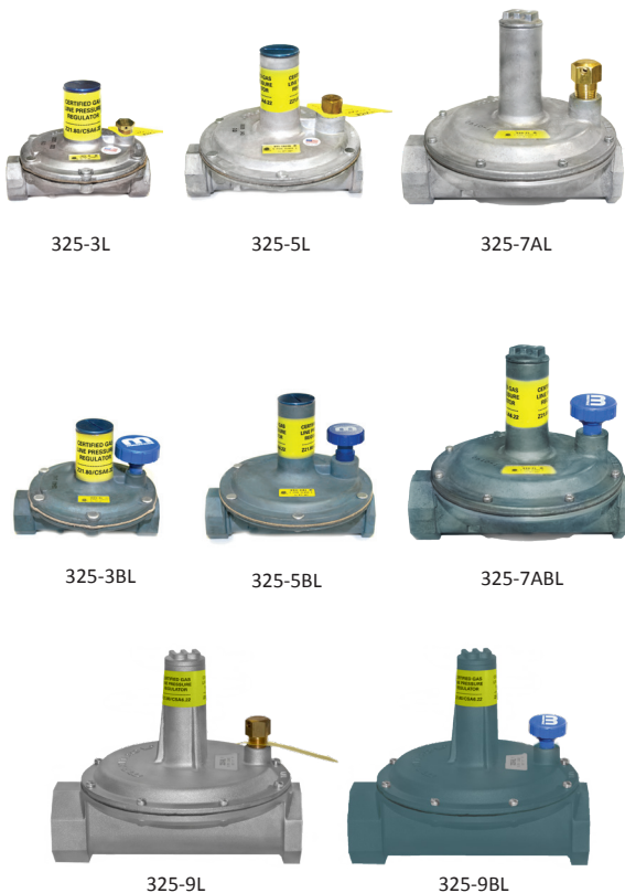
Figure 3: 325-L(B) Models: Pipe sizes from 3/8" to 2"
