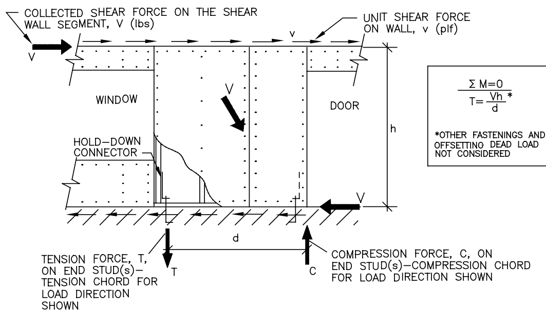
(a) DISCRETE HOLD-DOWN CONNECTOR FOR OVERTURNING RESTRAINT (SIMPLIFIED ANALYSIS)
